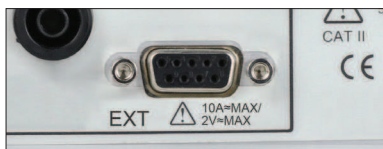
External sensor
